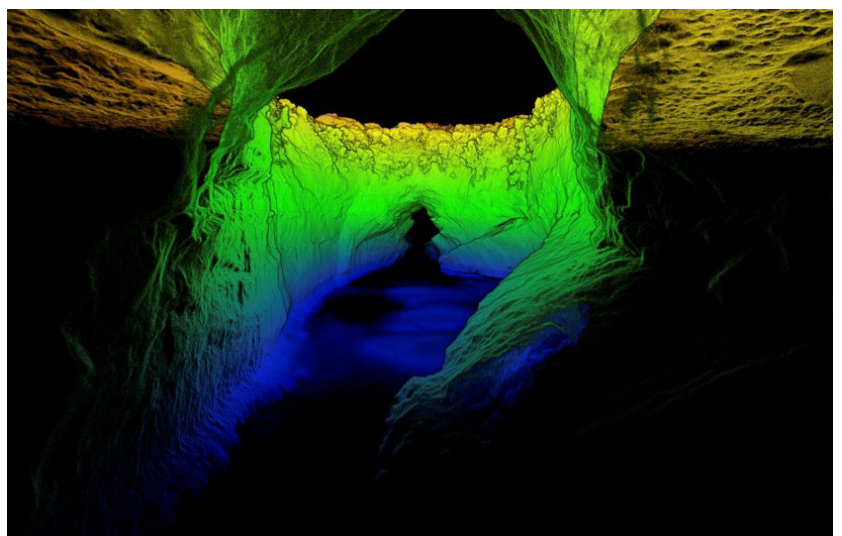
Development plans for the area around this blowhole, a natural formation that extends under the cliff, included the construction of a viewing platform. A 5-minute Hovermap flight captured data of the cliff and blowhole for the risk assessment and geotechnical inspection.
