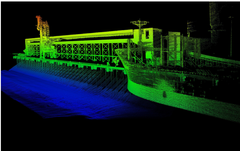
This port facility was comprehensively mapped above the pier with a flight and walking scans, and below with Hovermap on a craft. The point clouds were merged with an acoustic survey to form a complete asset data set.
