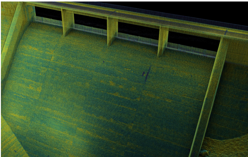
Hovermap adds LiDAR data capture to the traditional visual inspection of dams. Point clouds colored by intensity, as above, identify areas of deterioration and moisture seepage.
