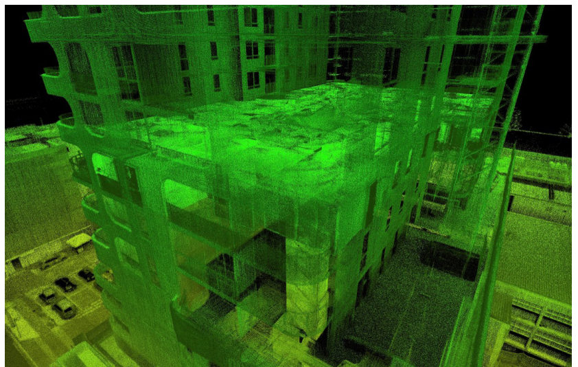
Construction sites contain many hazards for drones, but Hovermap is ideally suited to these complex environments. The details of this building were captured from flights and a walk through of the floors, merged to form a single data set.
