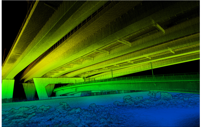
Bridge inspections are required throughout the entire bridge lifecycle. Flying a drone is the most time- and cost-effective way to scan these assets. Hovermap captures accurate data even when flying underneath the deck, where GPS may not always be available.
